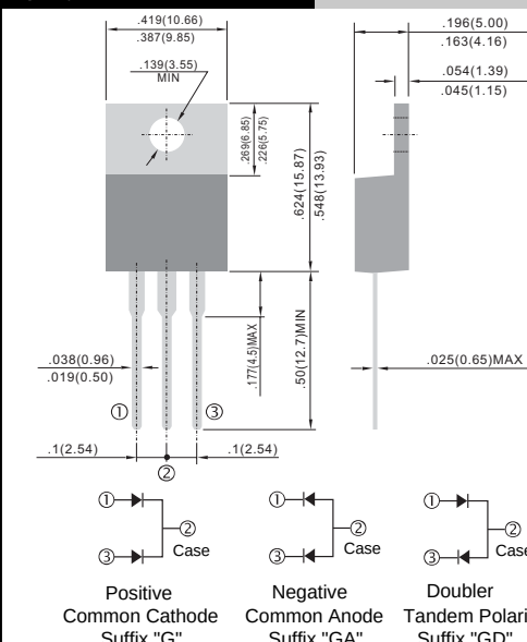
TO-220AB
