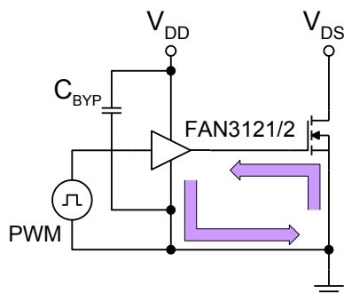
Figure 48. Current Path for MOSFET Turn-Off
