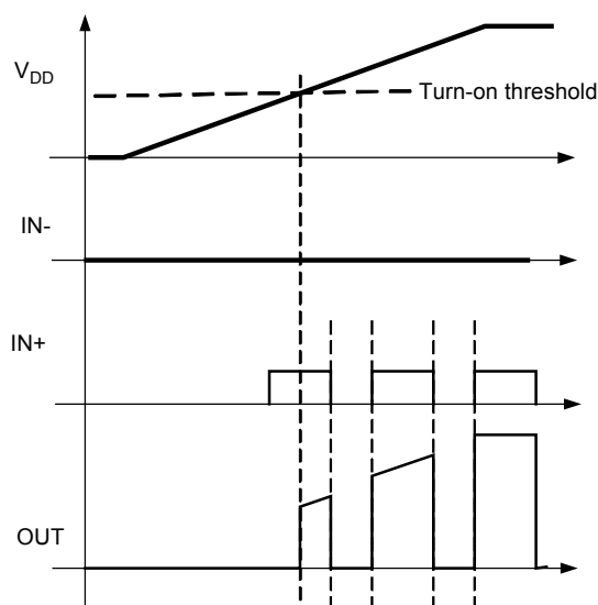
Figure 51. Non-Inverting Driver
