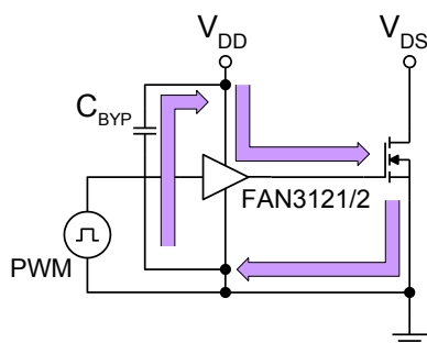
Figure 47. Current Path for MOSFET Turn-On
