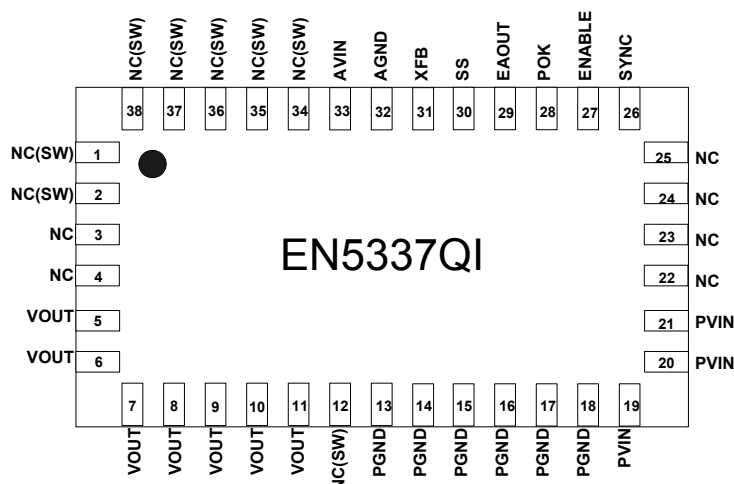
Figure 3: Pinout Diagram (Top View) NOTE: All perimeter pins must be soldered to PCB.
