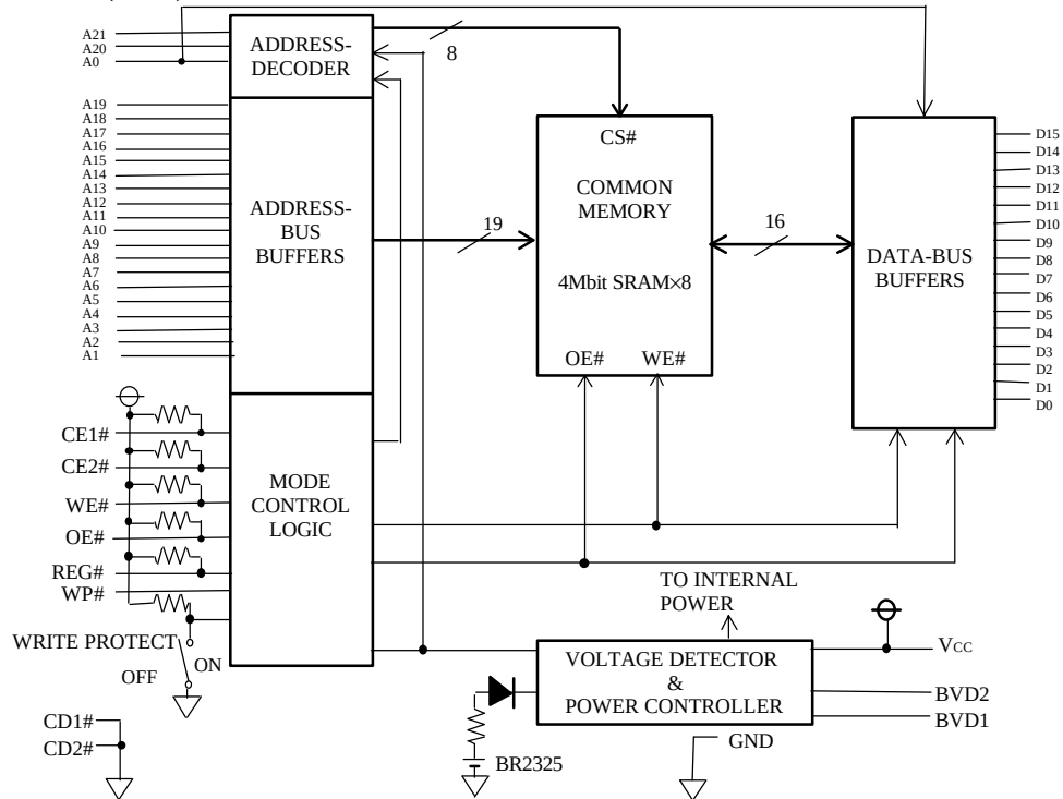
BLOCK DIAGRAM (4MB)
