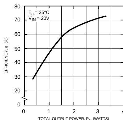
EFFICIENCY CHARACTERISTICS
