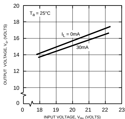
OUTPUT VOLTAGE VS INPUT VOLTAGE BETWEEN TERMINALS ⑩-⑨, ⑫-⑬, ⑭-⑮
