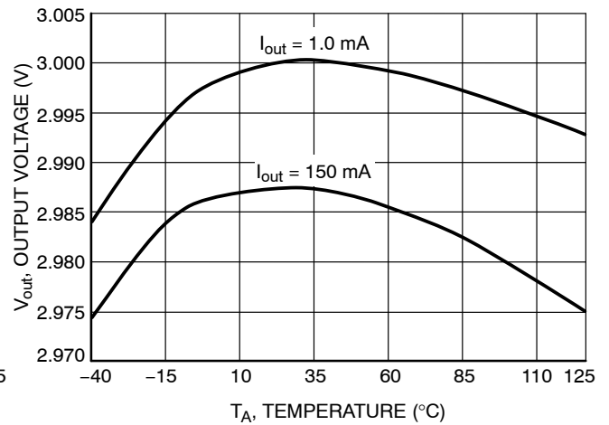
Figure 10. Output Voltage vs. Temperature ( 3.0\text{ V} Fixed Output, V_{in} = 6\text{ V} )
