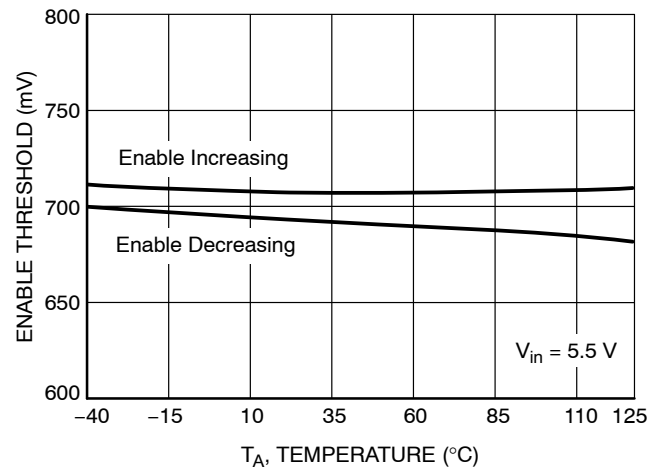
Figure 16. Enable Threshold vs. Temperature
