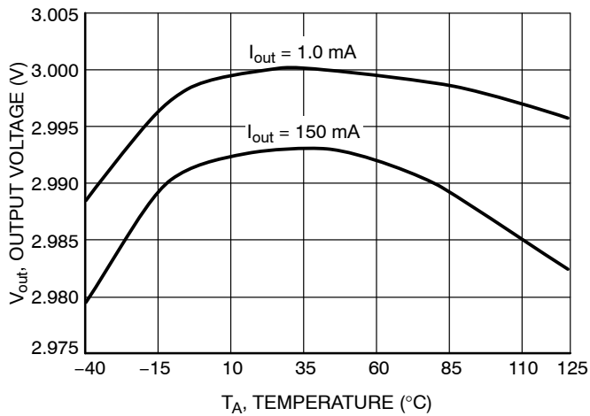
Figure 9. Output Voltage vs. Temperature ( 3.0\text{ V} Fixed Output, V_{in} = 3.5\text{ V} )
