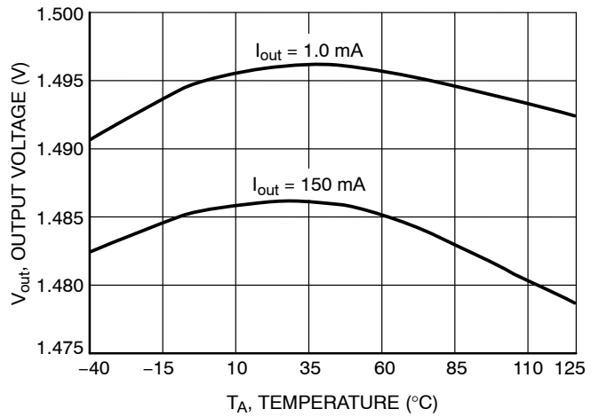
Figure 8. Output Voltage vs. Temperature ( 1.5\text{ V} Fixed Output, V_{in} = 6\text{ V} )
