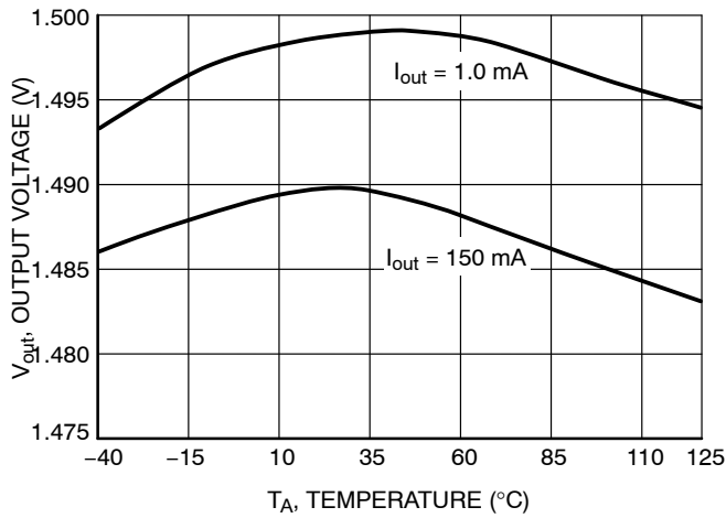
Figure 7. Output Voltage vs. Temperature ( 1.5\text{ V} Fixed Output, V_{in} = 2\text{ V} )
