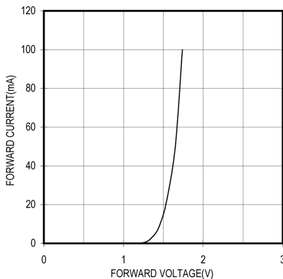
FORWARD I-V CHARACTERISTICS
