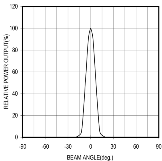
RADIATION PATTERN
