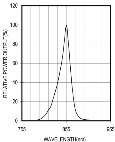
SPECTRAL OUTPUT
