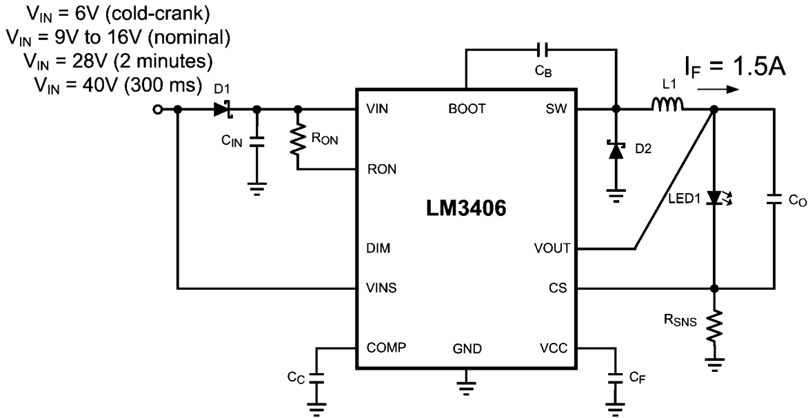
FIGURE 9. Schematic for Design Example 2
