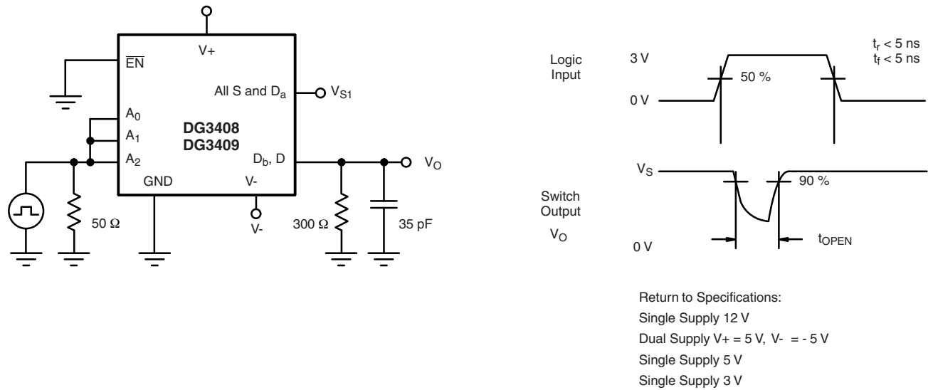
Figure 4. Break-Before-Make Interval
