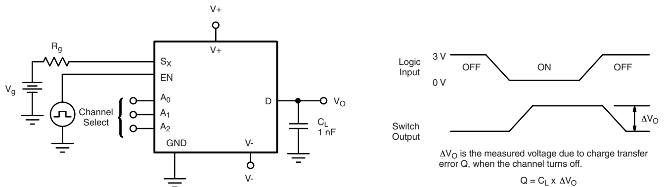
Figure 5. Charge Injection
