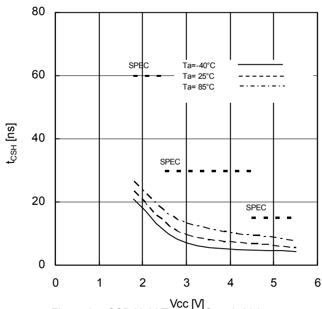
Figure 24. CSB Hold Time vs Supply Voltage
