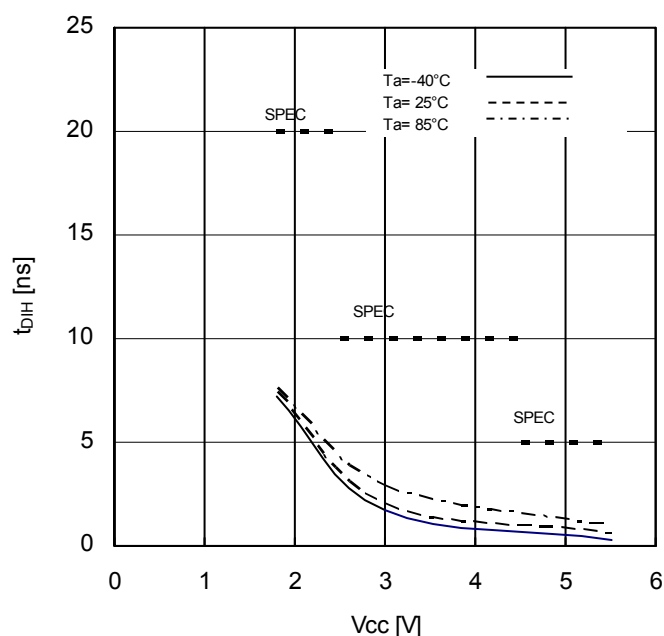
Figure 26. SI Hold Time vs Supply Voltage
