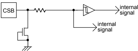
Figure 52. CSB input equivalent circuit
