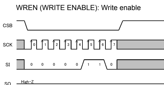
Figure 36. Write enable command
