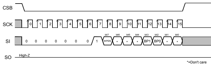
Figure 40. Write status register
