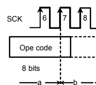
Figure 47. WREN/WRDI cancel valid timing
