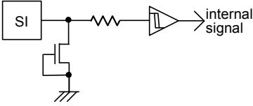
Figure 54. SI input equivalent circuit
