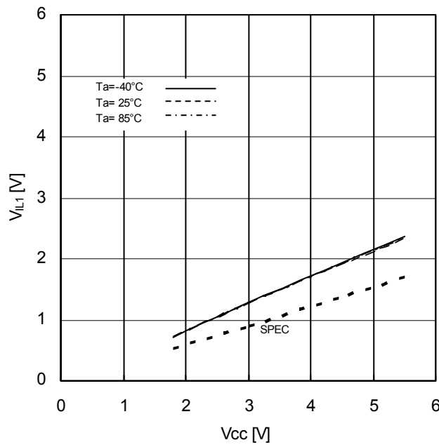
Figure 6. Input Low Voltage1 vs Supply Voltage (CSB,SCK,SI,HOLDB,WPB)
