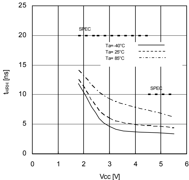
Figure 30. HOLDB Release Hold Time vs Supply Voltage
