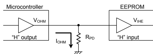
Figure 49. Pull down resistance
