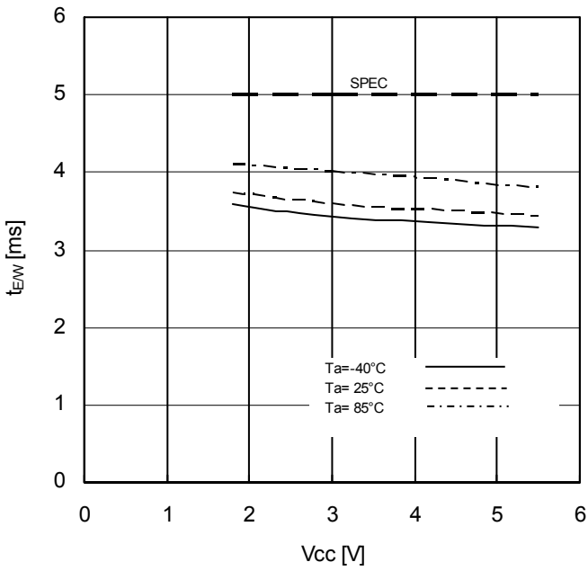
Figure 35. Write Cycle Time vs Supply Voltage
