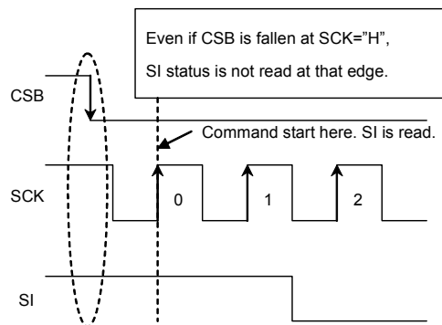
Figure 58. Operating timing
