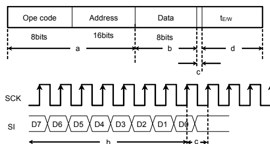
Figure 45. WRITE cancel valid timing
