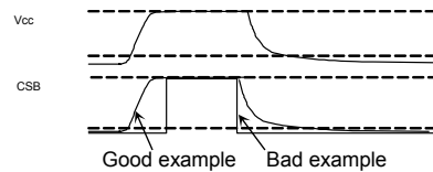
Figure 57. CSB timing at power ON/OFF
