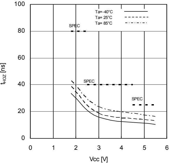
Figure 31. Time from HOLDB to Output High-Z vs Supply Voltage
