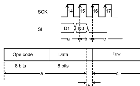
Figure 46. WRSR cancel valid timing
