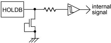
Figure 55. HOLDB input equivalent circuit
