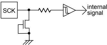
Figure 53. SCK input equivalent circuit
