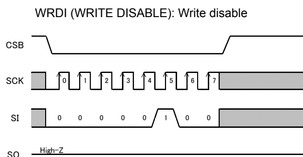
Figure 37. Write disable command
