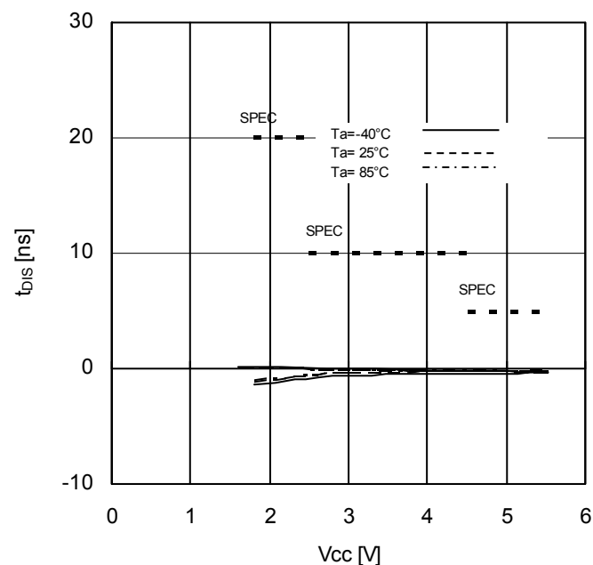
Figure 25. SI Setup Time vs Supply Voltage
