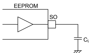
Figure 50. SO load capacity
