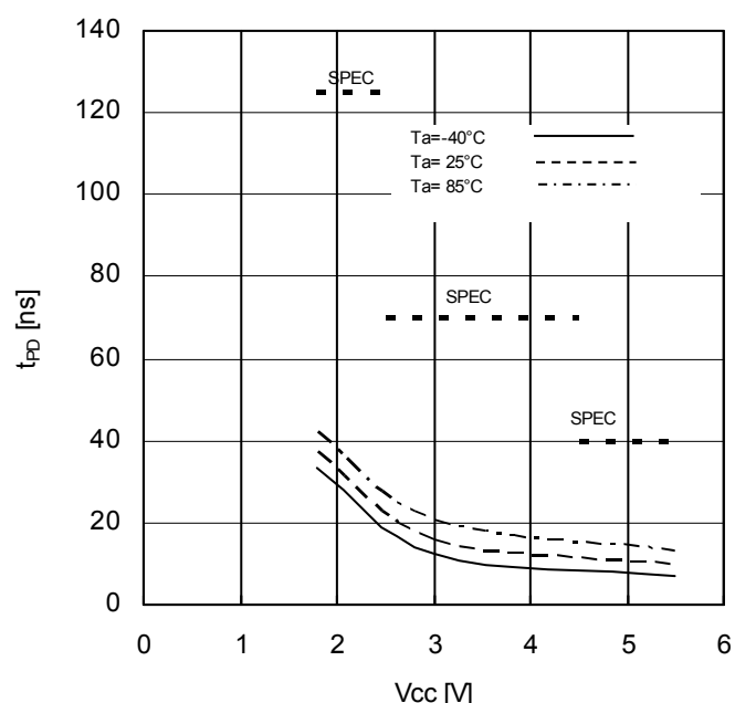
Figure 27. Data Output Delay Time vs Supply Voltage
