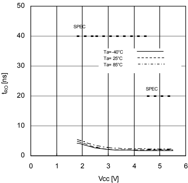
Figure 33. OUTPUT Rise Time vs Supply Voltage
