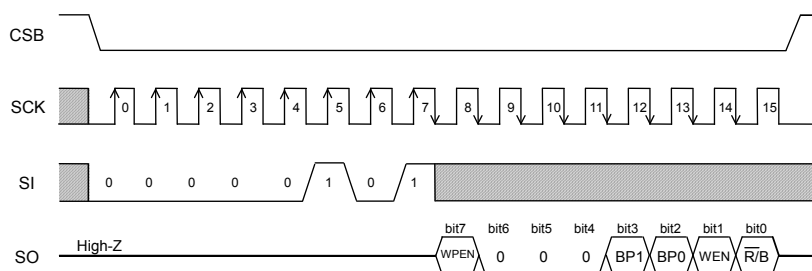
Figure 41. Read status register command
