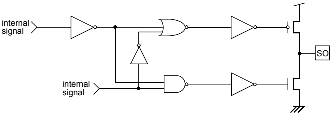
Figure 51. SO output equivalent circuit
