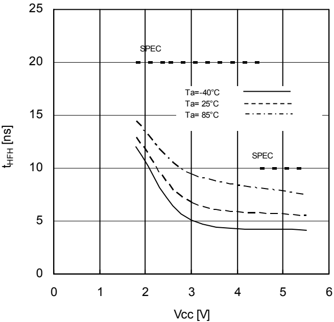
Figure 29. HOLDB Setting Hold Time vs Supply Voltage
