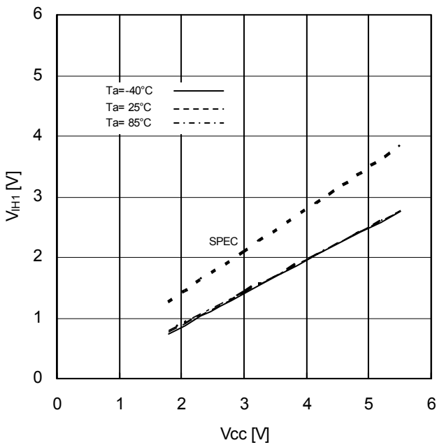
Figure 5. Input High Voltage1 vs Supply Voltage (CSB,SCK,SI,HOLDB,WPB)
