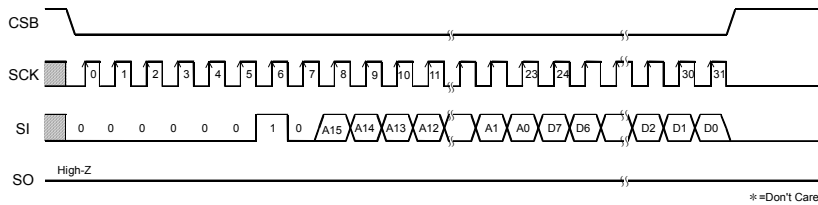
Figure 39. Write command
