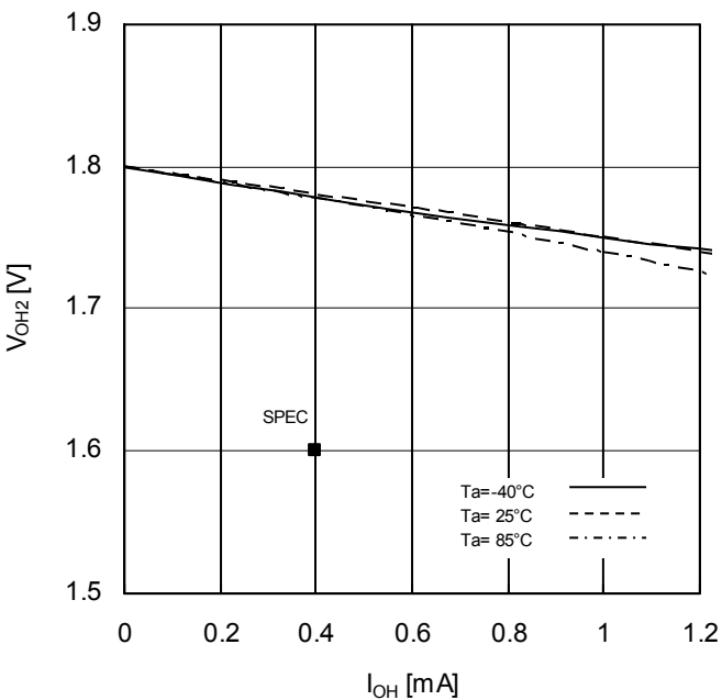
Figure 10. Output High Voltage2 vs Output Current (Vcc=1.8V)
