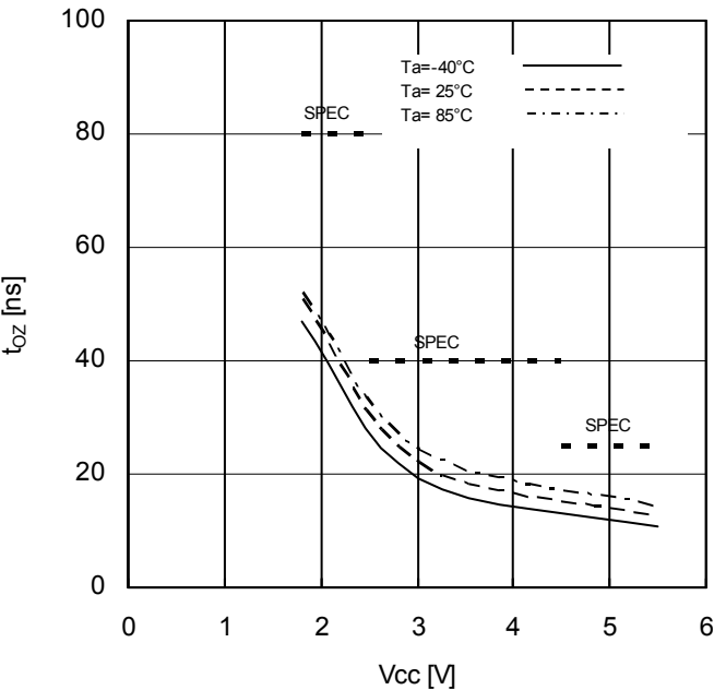
Figure 28. Output Disable Time vs Supply Voltage
