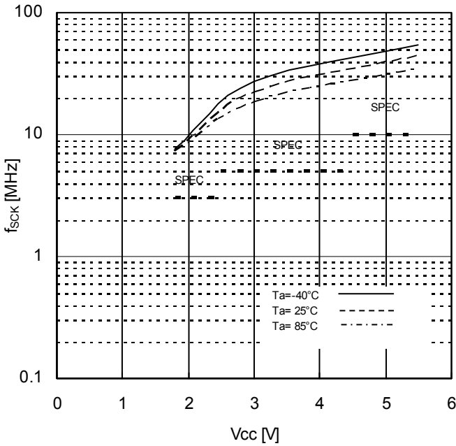
Figure 19. SCK Frequency vs Supply Voltage
