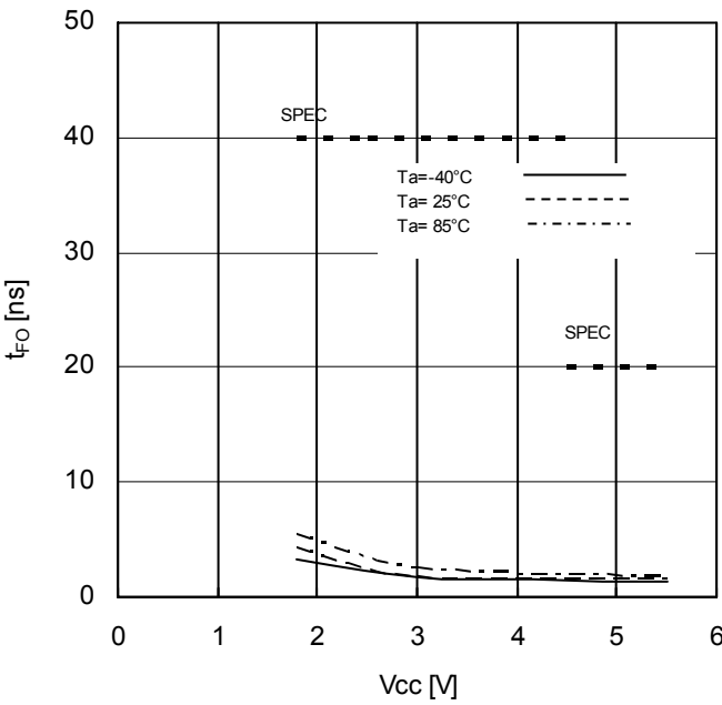
Figure 34. OUTPUT Fall Time vs Supply Voltage
