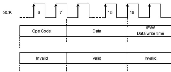
Figure 42. WPB valid timing (At inputting WRSR command)
