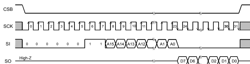
Figure 38. Read command
