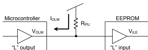
Figure 48. Pull up resistance
