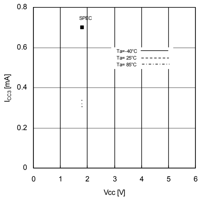
Figure 15. Supply Current (Read) vs Supply Voltage (fSCK=3MHz)
