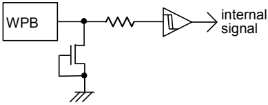
Figure 56. WPB input equivalent circuit
