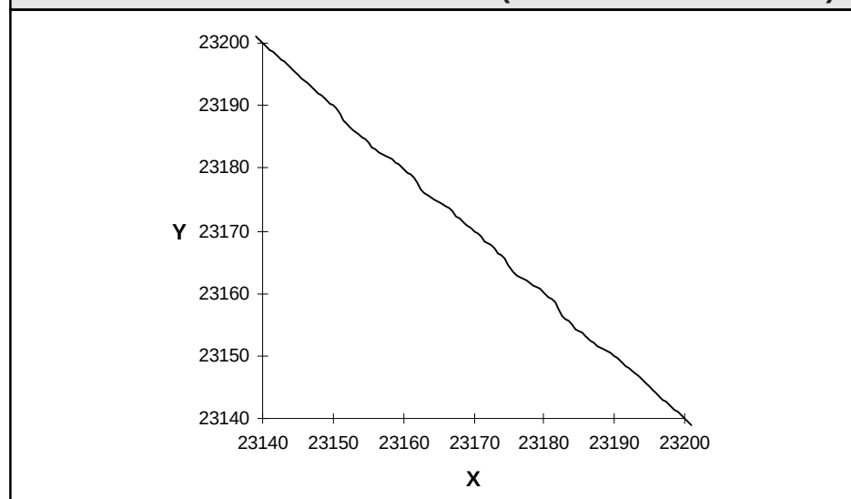
FIGURE 3. CIRCLE TEST RESULT NEAR 45^\circ (16-BIT INTERNAL PROCESSOR)
