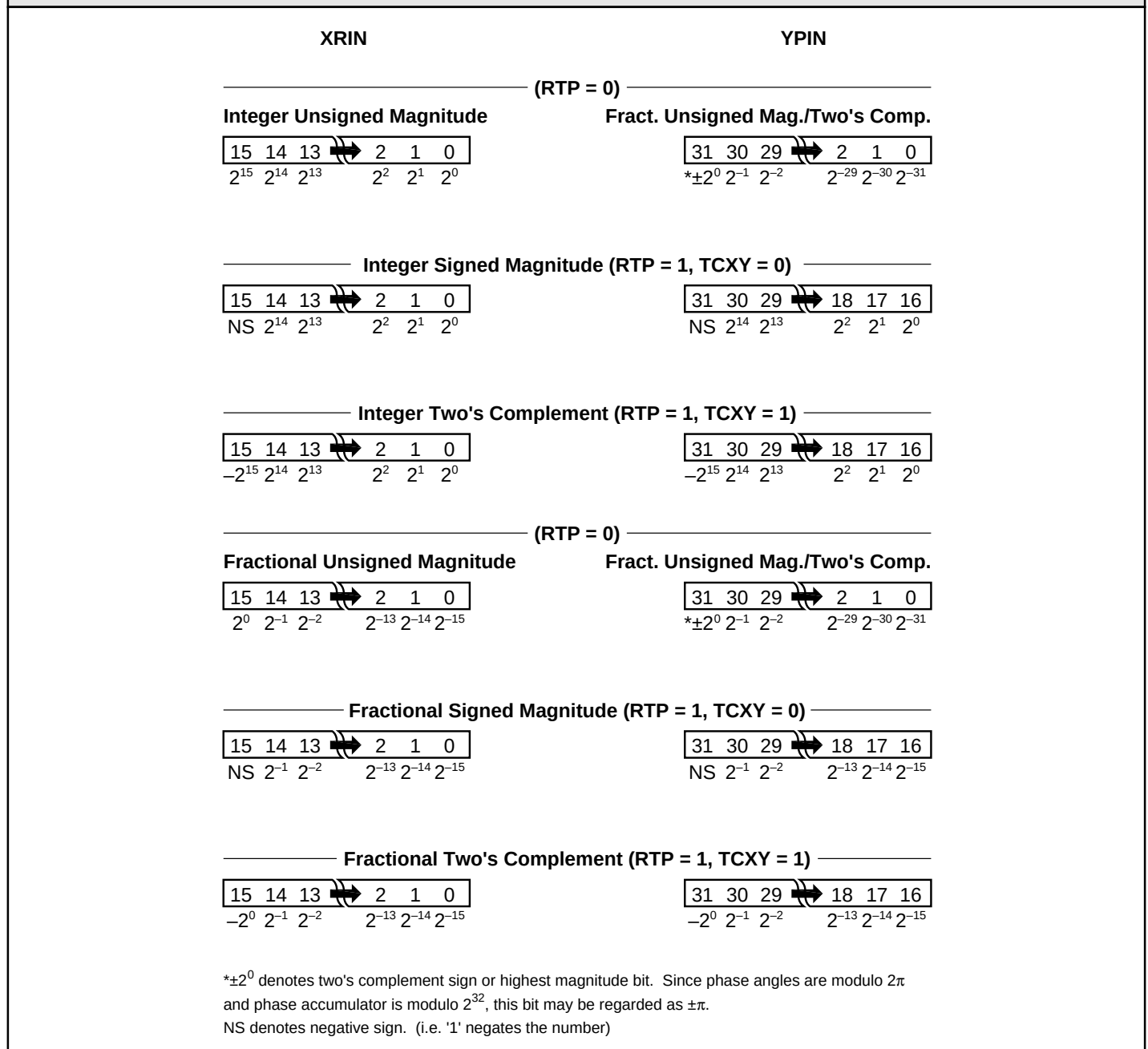
FIGURE 1A. INPUT FORMATS
