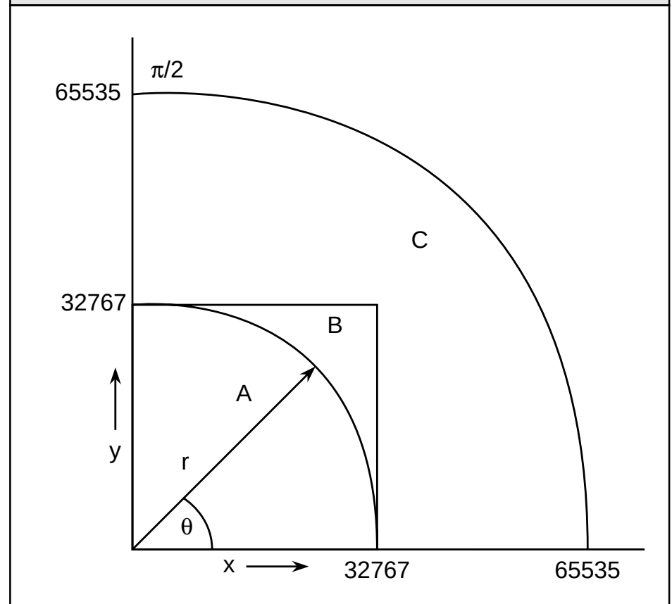
FIGURE 2. CONVERSION RANGES
