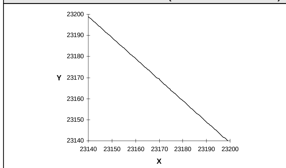
FIGURE 4. CIRCLE TEST RESULT NEAR 45^\circ (24-BIT INTERNAL PROCESSOR)
