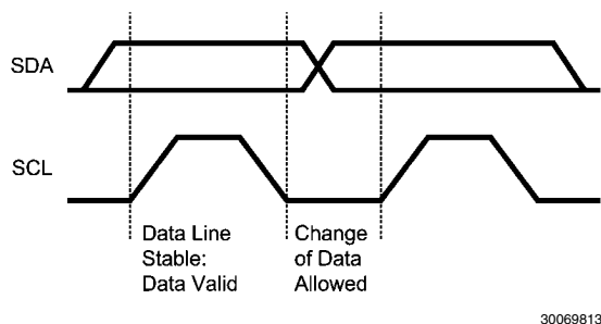
FIGURE 10. Bit Transfer
