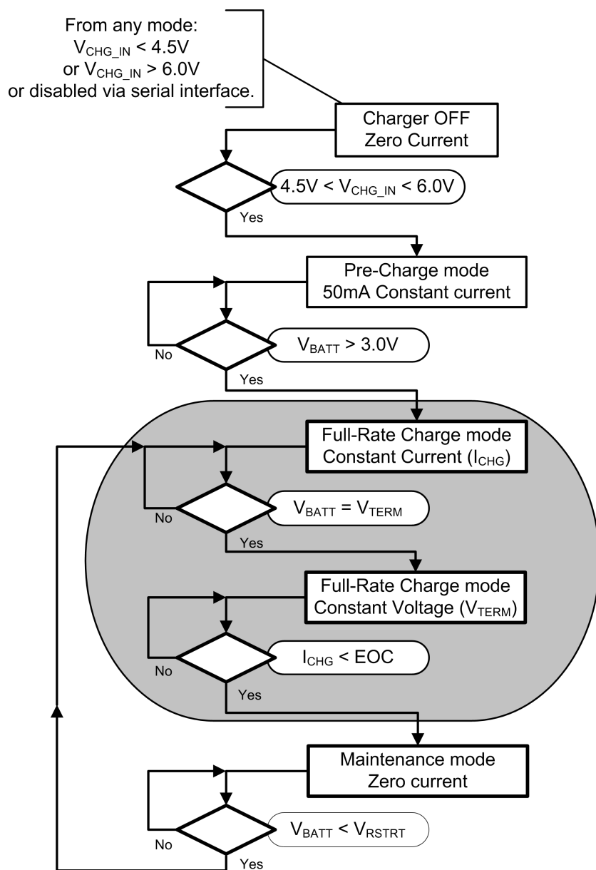
FIGURE 5. Simplified Charger Functional State Diagram (EOC is enabled)
