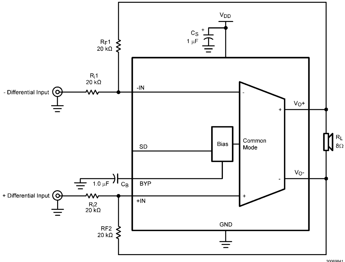
FIGURE 9. Audio Block
