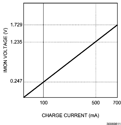
FIGURE 7. IMON Voltage vs. Charge Current
