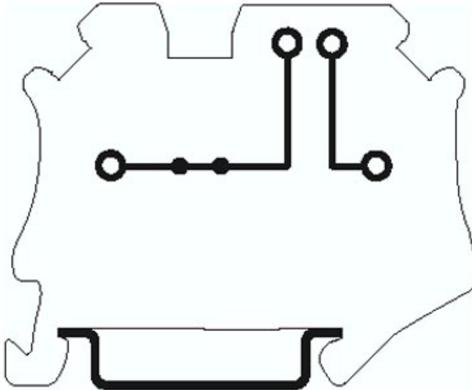
Circuit diagram
