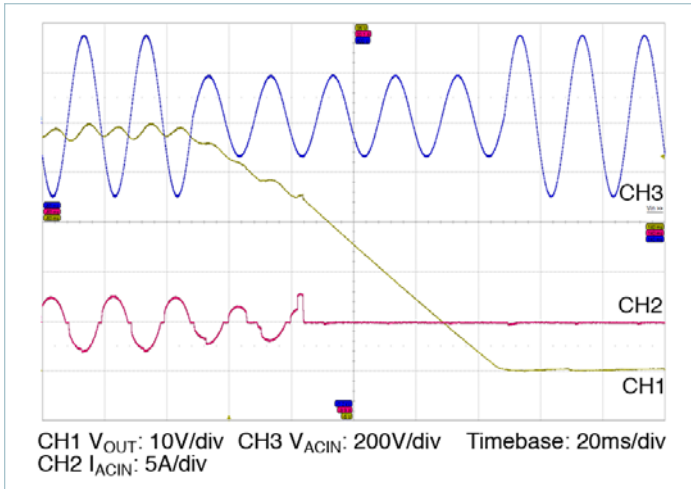
Figure 9 — 230V, 120V range change transient response 16.7A, I_{OUT} = 8.3\text{A} , C_{OUT} = 10,000\mu\text{F}
