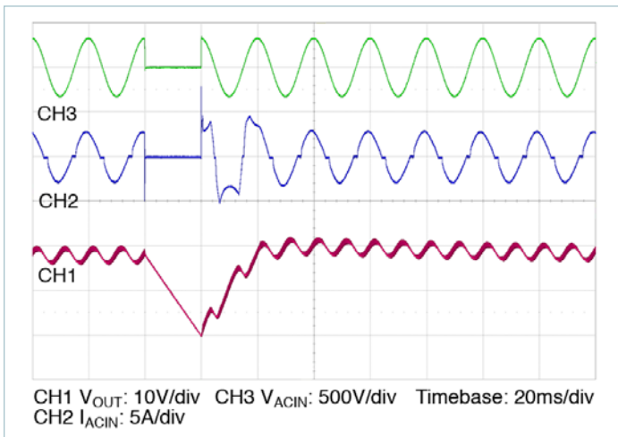
Figure 11 — Line drop out, 230V 50Hz, 90° phase, V_{IN} = 230\text{V} , 50Hz, I_{OUT} = 8.3\text{A} , C_{OUT} = 10,000\mu\text{F}
