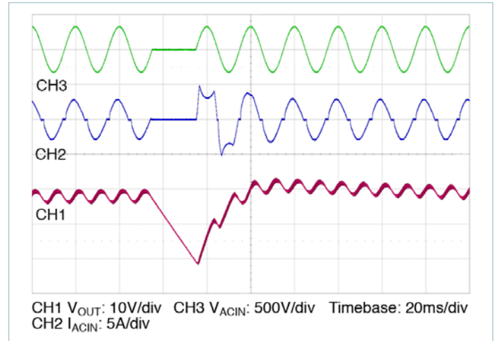
Figure 10 — Line drop out, 230V 50Hz, 0° phase, I_{OUT} = 8.3\text{A} , C_{OUT} = 10,000\mu\text{F}
