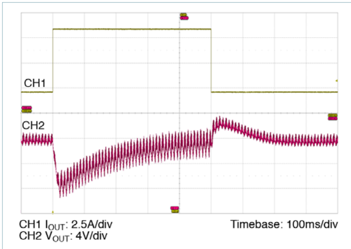
Figure 7 — Typical output voltage transient response, T_{CASE} = 30^{\circ}\text{C} , V_{IN} = 230\text{V} , I_{OUT} = 8.3\text{A} , 2.1A C_{OUT} = 10,000\mu\text{F}
