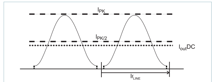
Figure 22 — Output current waveform
