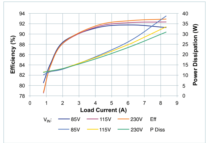
Figure 18 — V_{IN} to V_{OUT} efficiency and power dissipation vs. V_{IN} and I_{OUT} , T_{CASE} = 25^{\circ}\text{C}
