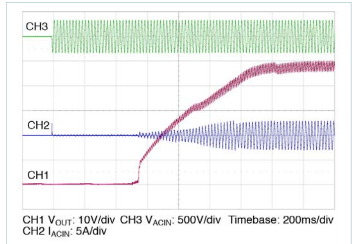
Figure 8 — Typical startup waveform, application of V_{IN} , R_{LOAD} = 5.7\Omega , C_{OUT} = 10,000\mu\text{F}
