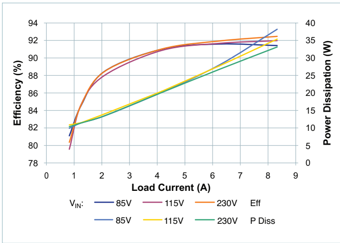
Figure 17 — V_{IN} to V_{OUT} efficiency and power dissipation vs. V_{IN} and I_{OUT} , T_{CASE} = -40^{\circ}\text{C}
