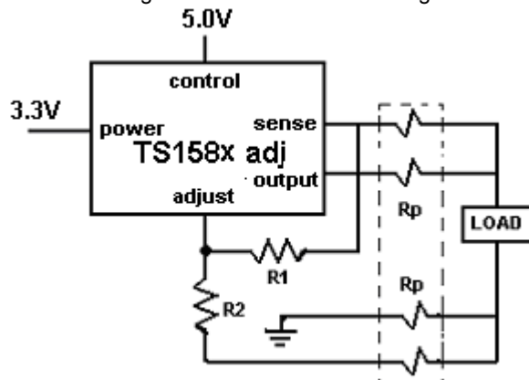
Figure 2. Remote Load Sensing
