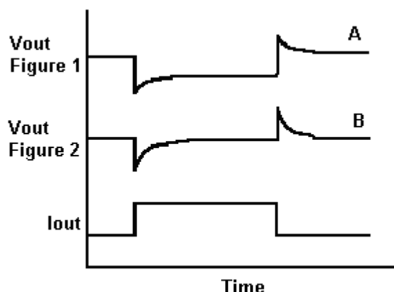
Figure 3. Remote Sensing Improves Load Regulation
