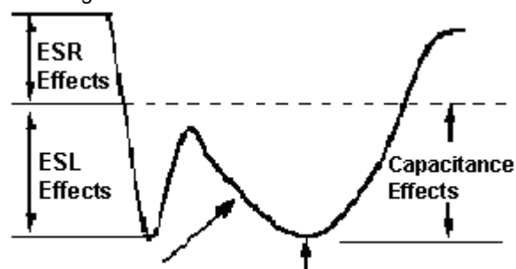
Figure 4. illustrates there transient effects.
