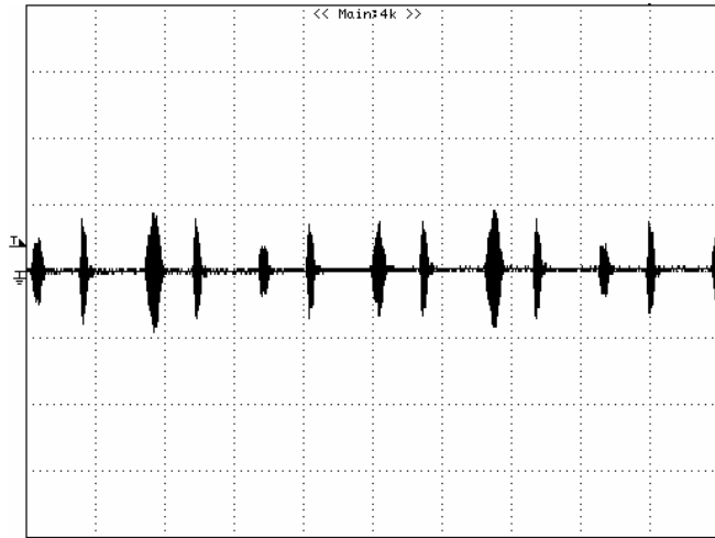
Figure 12: Input reflected ripple current, i_s , through a 12\mu\text{H} source inductor at nominal input voltage and rated load current (100 mA/div, 2\mu\text{s}/\text{div} )
