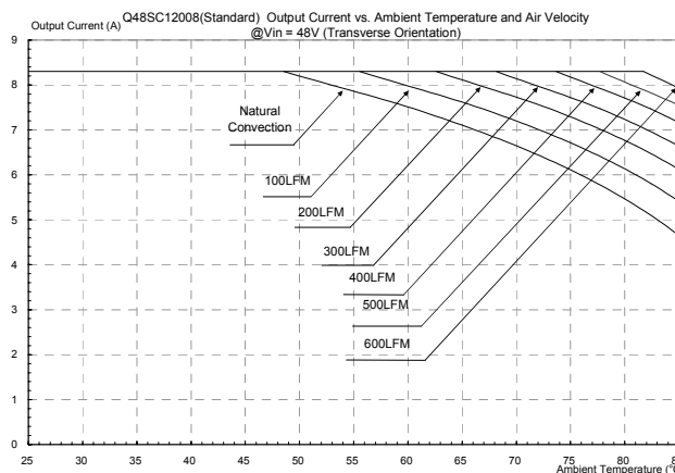
Figure 22: Output current vs. ambient temperature and air velocity@Vin=48V (Transverse Orientation, Airflow from Vin+ to Vin-)
