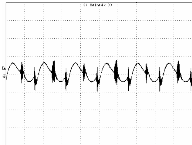
Figure 14: Output voltage ripple at nominal input voltage and rated load current ( I_o=8.3\text{A} ) ( 20\text{mV}/\text{div} , 2\mu\text{s}/\text{div} ) Load capacitance: 1\mu\text{F} ceramic capacitor and 10\mu\text{F} tantalum capacitor. Bandwidth: 20 MHz. Scope measurements should be made using a BNC cable (length shorter than 20 inches). Position the load between 51 mm to 76 mm (2 inches to 3 inches) from the module.
