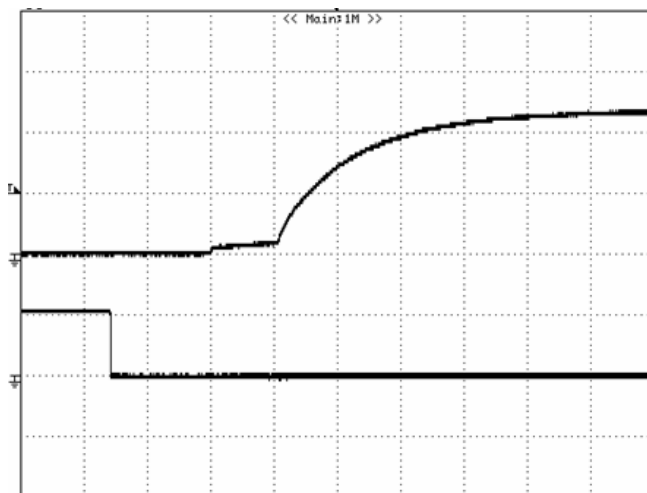
Figure 5: Turn-on transient at zero load current (2ms/div). V_{in}=48V . Top Trace: V_{out} , 5V/div; Bottom Trace: ON/OFF input, 5V/div
