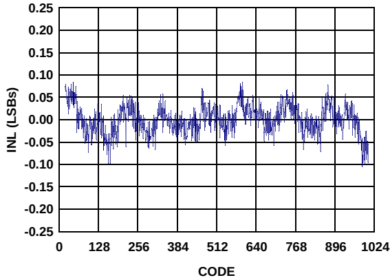
FIGURE 12. INTEGRAL NONLINEARITY
