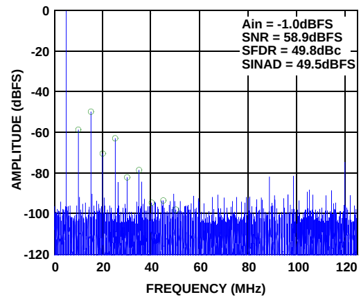
FIGURE 19. SINGLE-TONE SPECTRUM @ 995MHz
