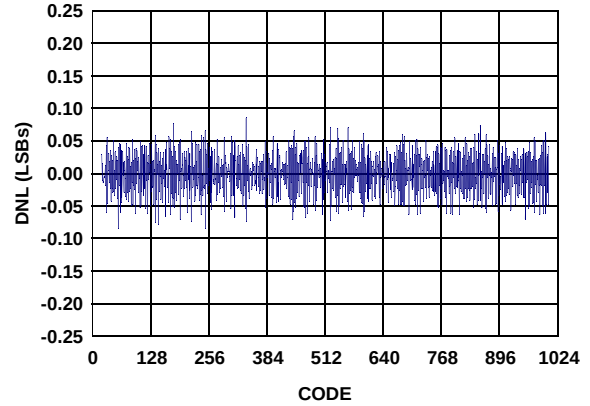
FIGURE 11. DIFFERENTIAL NONLINEARITY
