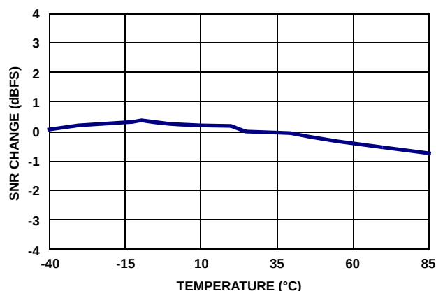
FIGURE 24. SNR PERFORMANCE vs TEMPERATURE AFTER +25°C CALIBRATION
