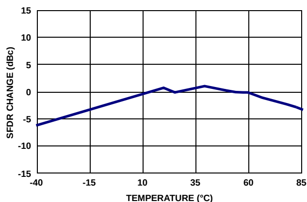
FIGURE 25. SFDR PERFORMANCE vs TEMPERATURE AFTER +25°C CALIBRATION
