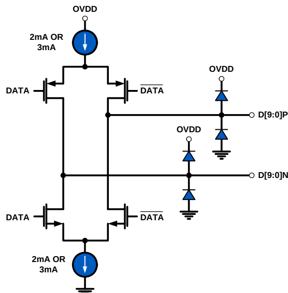
FIGURE 45. LVDS OUTPUTS
