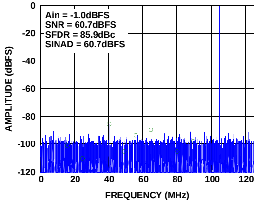
FIGURE 16. SINGLE-TONE SPECTRUM @ 105MHz
