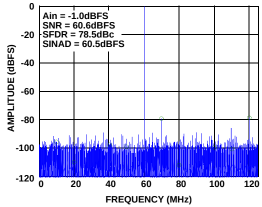
FIGURE 17. SINGLE-TONE SPECTRUM @ 190MHz
