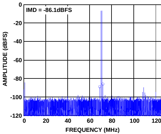
FIGURE 20. TWO-TONE SPECTRUM @ 70MHz
