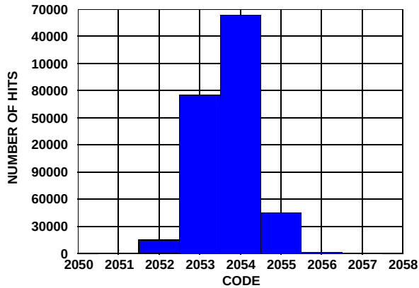
FIGURE 14. NOISE HISTOGRAM
