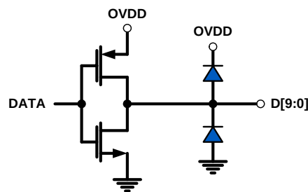
FIGURE 46. CMOS OUTPUTS
