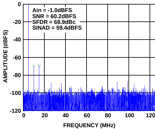
FIGURE 18. SINGLE-TONE SPECTRUM @ 495MHz
