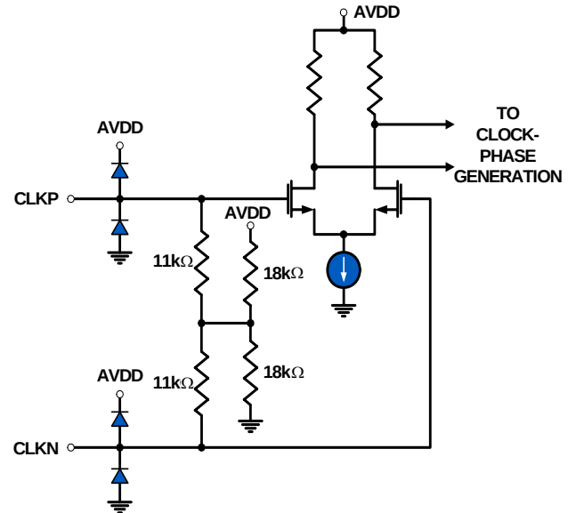
FIGURE 42. CLOCK INPUTS
