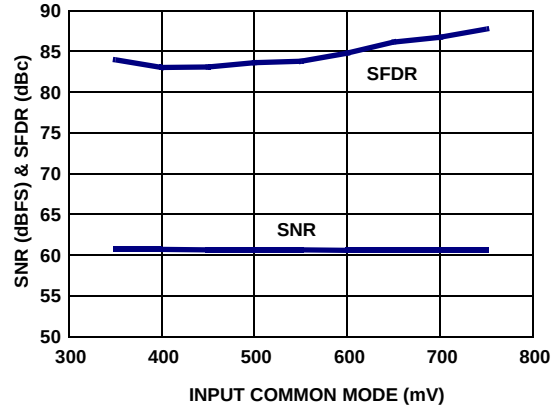
FIGURE 13. SNR AND SFDR vs VCM
