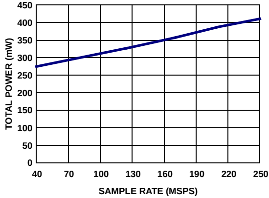
FIGURE 10. POWER vs f_{SAMPLE} IN 3mA LVDS MODE
