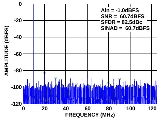
FIGURE 15. SINGLE-TONE SPECTRUM @ 10MHz
