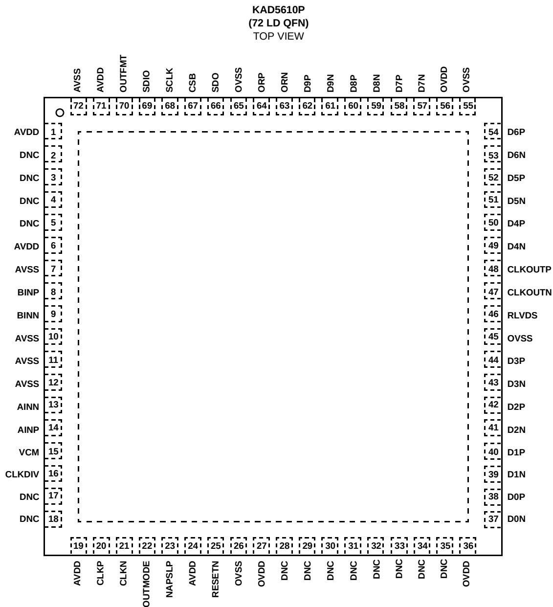
FIGURE 3. PIN CONFIGURATION
