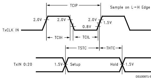
FIGURE 6. DS90CR217 (Transmitter) Setup/Hold and High/Low Times
