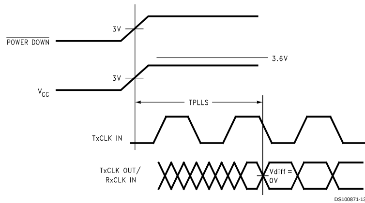
FIGURE 10. DS90CR217 (Transmitter) Phase Lock Loop Set Time
