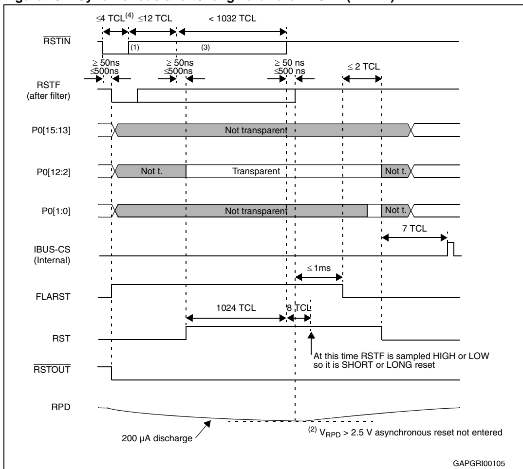
Figure 28. Synchronous short / long hardware RESET (EA = 1)
