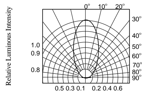
FIG.6 RADIATION DIAGRAM
