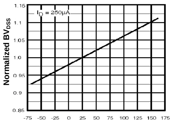
Figure 3. Max BV_{DS} vs Junction Temperature
