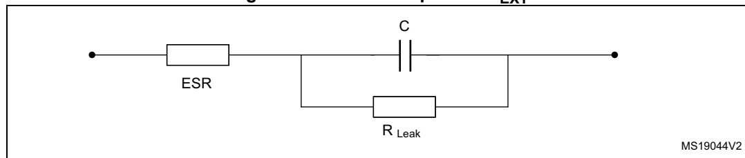
Figure 29. External capacitor C_{\text{EXT}}
