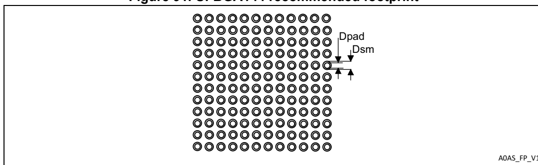
Figure 91. UFBGA144 recommended footprint
