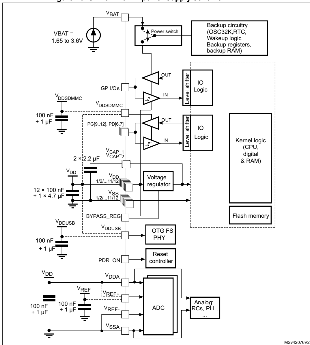
Figure 26. STM32F732xx power supply scheme
