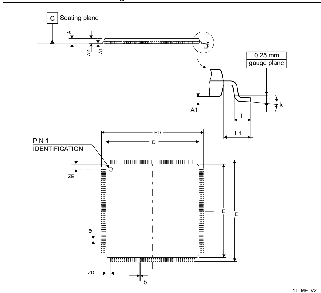
Figure 87. LQFP176 outline
