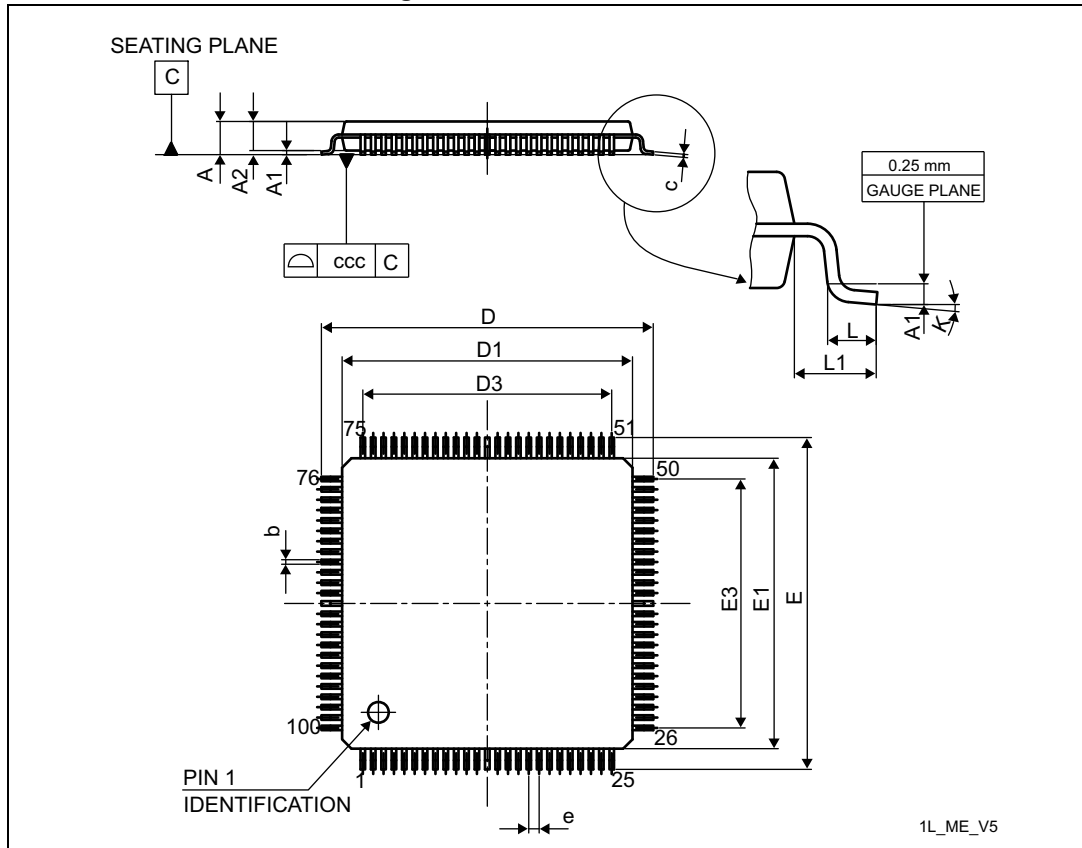
Figure 81. LQFP100 outline
