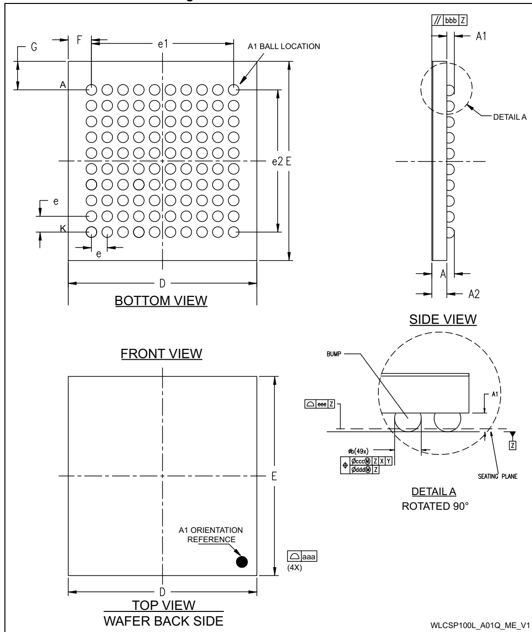
Figure 96. WLCSP100 outline
