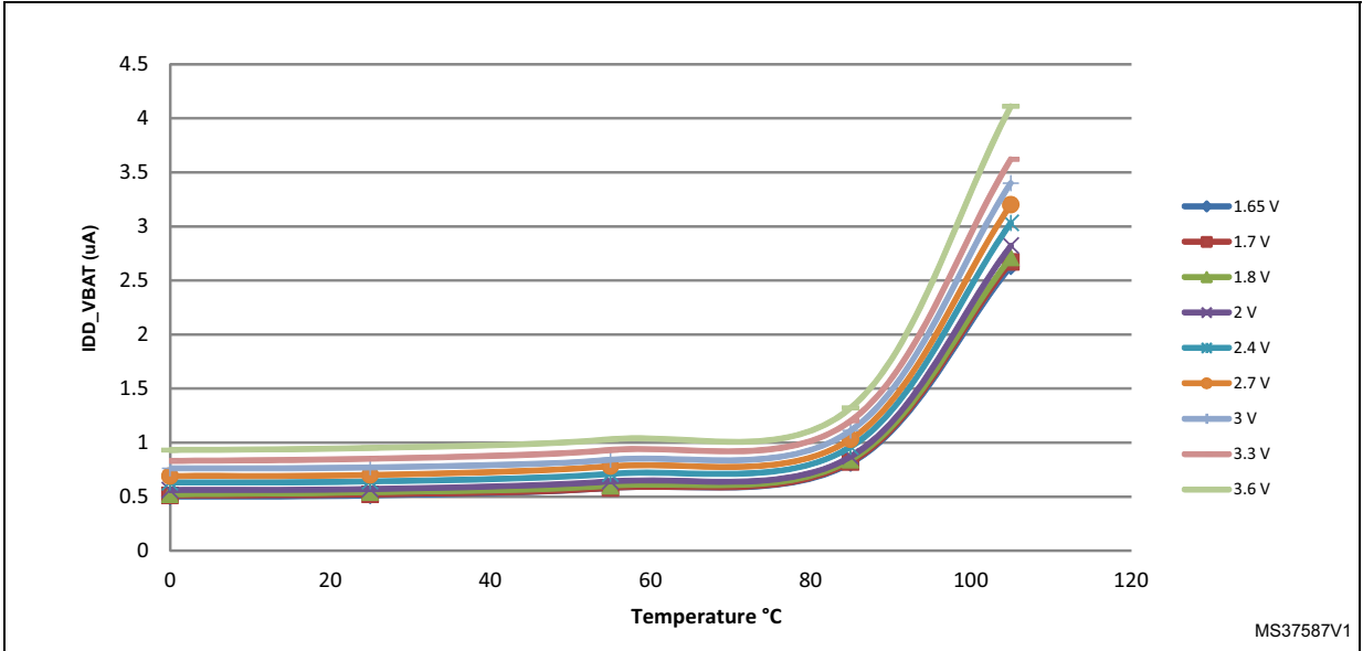
Figure 32. Typical V_{BAT} current consumption (RTC ON/BKP SRAM OFF and LSE in medium high drive mode)
