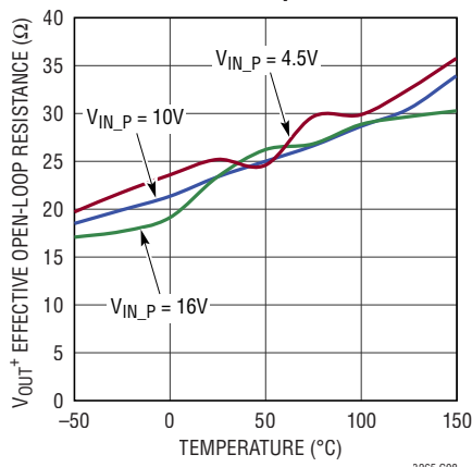
V_{OUT^+} Effective Open-Loop Resistance vs Temperature
