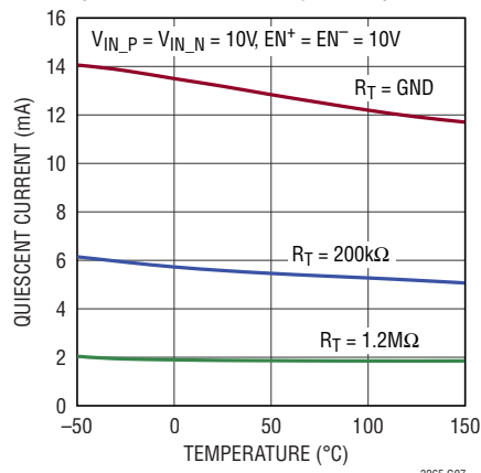
Quiescent Current vs Temperature (Constant Frequency Mode)
