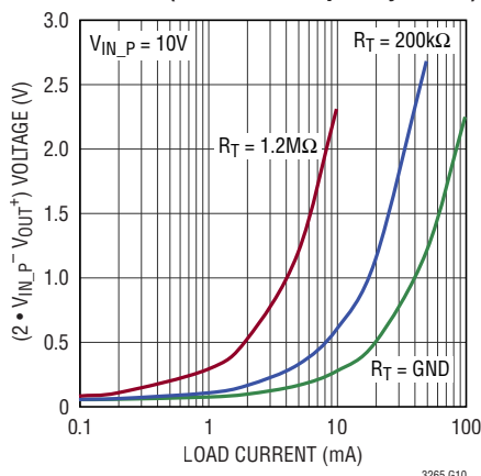
V_{OUT^+} Voltage Loss vs Output Current (Constant Frequency Mode)
