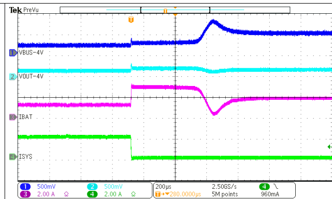
图 57. IBAT Regulation During Load Step Down
