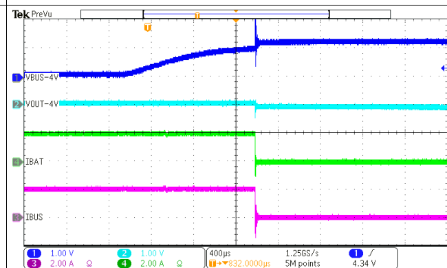
图 59. IBUS OCP During Load Transient
