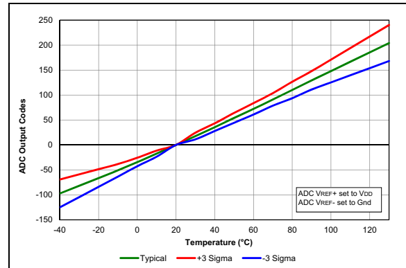
FIGURE 38-46: Temp. Indicator Slope Normalized to 20^\circ C , High Range, V_{DD} = 3.0V .
