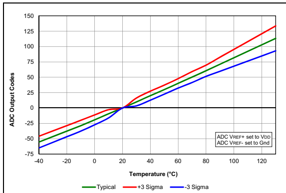
FIGURE 38-44: Temp. Indicator Slope Normalized to 20^\circ C , High Range, V_{DD} = 5.5V , PIC16F18857/77 Only.
