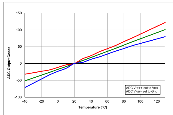
FIGURE 38-48: Temp. Indicator Slope Normalized to 20^\circ C , Low Range, V_{DD} = 3.0V .
