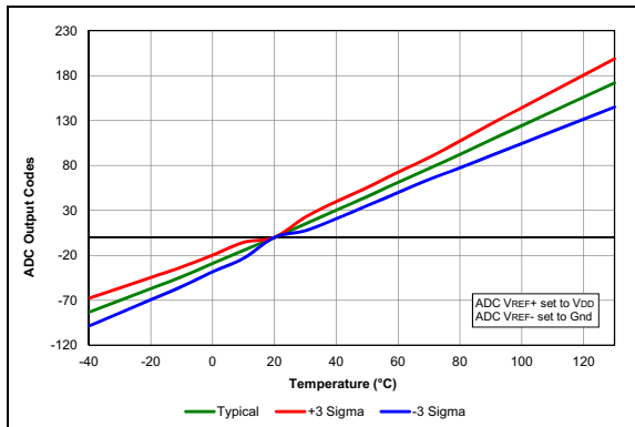
FIGURE 38-45: Temp. Indicator Slope Normalized to 20^\circ C , High Range, V_{DD} = 3.6V .
