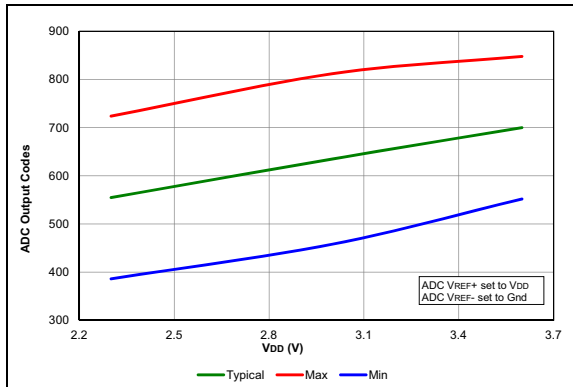
FIGURE 38-43: Temp. Indicator Initial Offset, Low Range, Temp. = 20^\circ C , PIC16LF18857/77 Only.
