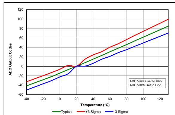
FIGURE 38-47: Temp. Indicator Slope Normalized to 20^\circ C , Low Range, V_{DD} = 3.6V .
