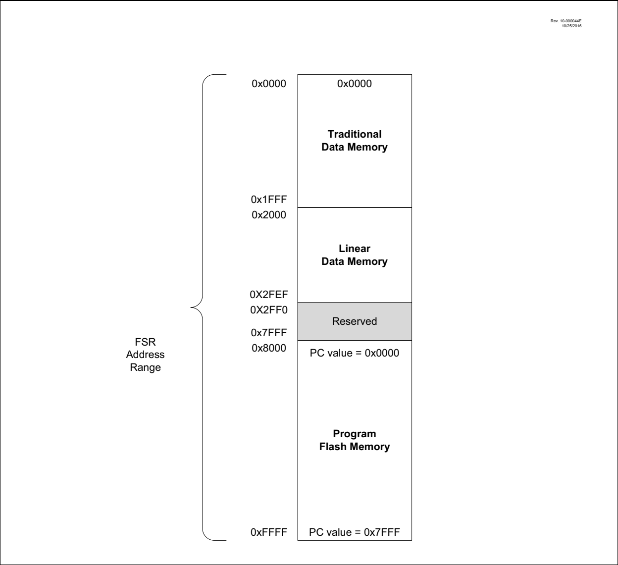
FIGURE 3-8: INDIRECT ADDRESSING
