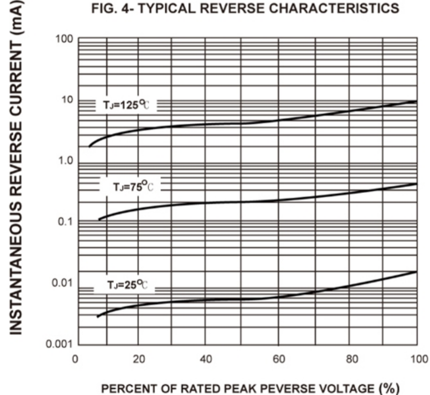
FIG. 4- TYPICAL REVERSE CHARACTERISTICS
