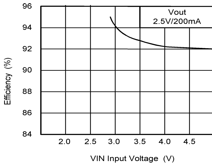
AT1392 Efficiency
