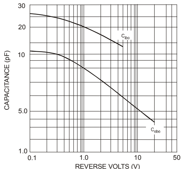
Fig. 1 Typical Capacitance (4401)
