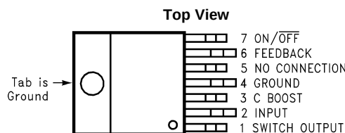
Figure 2. TO-220 Package See Package Number NDZ0007B
