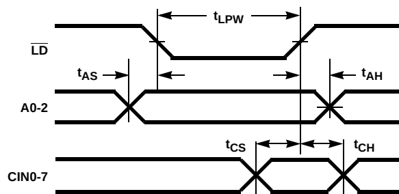
FIGURE 5. CONFIGURATION TIMING
