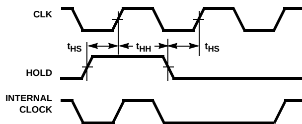
FIGURE 7. HOLD TIMING
