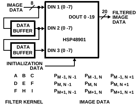
FIGURE 3. 3 \times 3 KERNEL ON AN 8-BIT IMAGE
