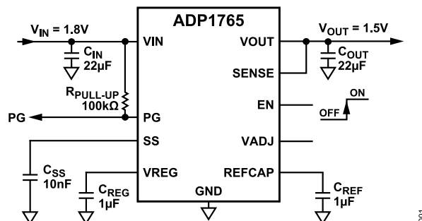
Figure 1. Fixed Output Operation
