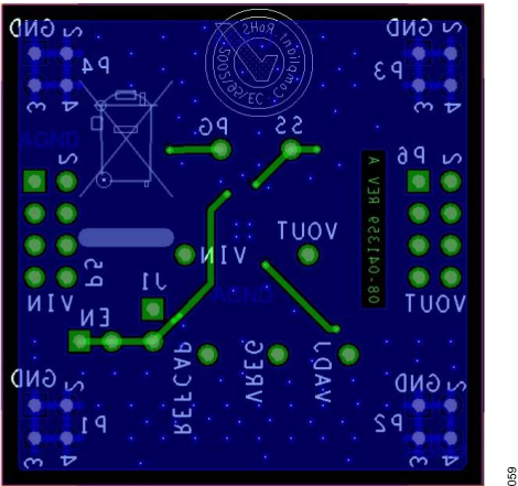
Figure 59. Typical Board Layout, Bottom Side
