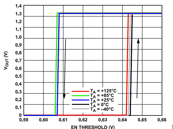
Figure 43. Output Voltage ( V_{OUT} ) vs. EN Threshold, V_{OUT} = 1.3 V
