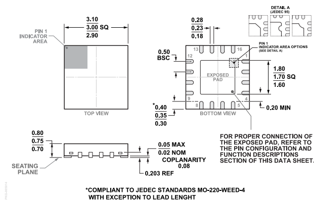
Figure 60. 16-Lead Lead Frame Chip Scale Package [LFCSP] 3 mm x 3 mm Body and 0.75 mm Package Height (CP-16-48) Dimensions shown in millimeters
