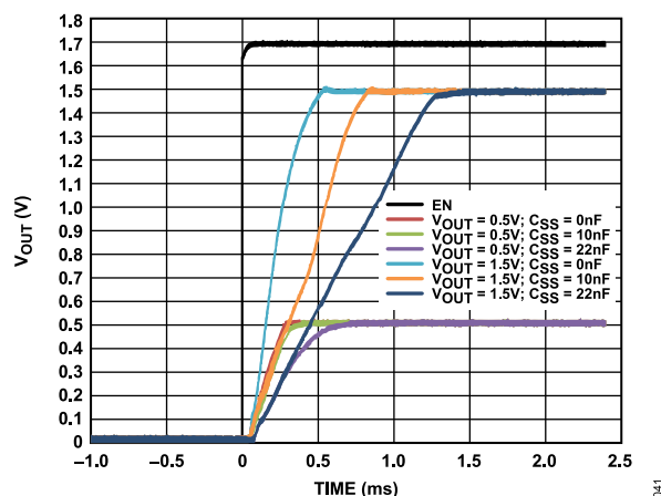
Figure 41. Adjustable V_{OUT} Ramp-Up with External Soft Start Capacitor ( V_{OUT, EN} ) vs. Time
