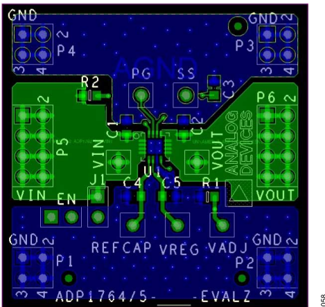
Figure 58. Typical Board Layout, Top Side
