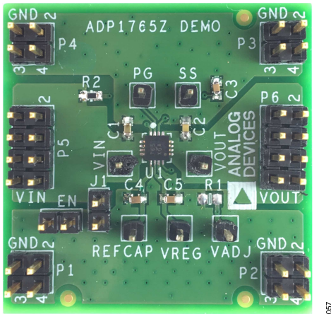
Figure 57. Evaluation Board
