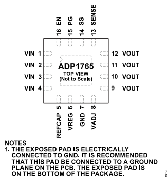
Figure 3. Pin Configuration
