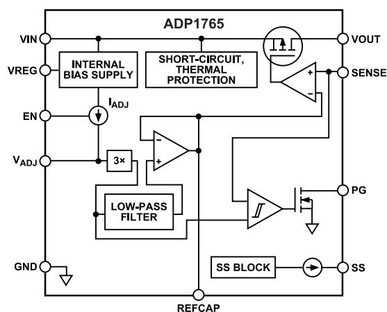
Figure 39. Functional Block Diagram, Adjustable Output
