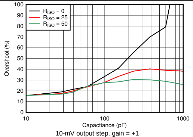
图 30. Small Signal Overshoot vs Capacitive Load
