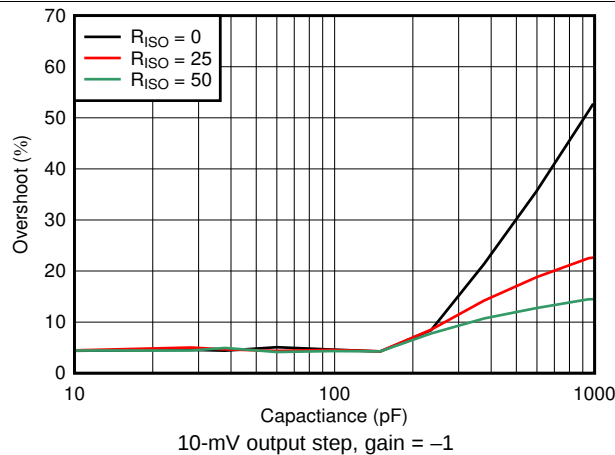
图 29. Small Signal Overshoot vs Capacitive Load
