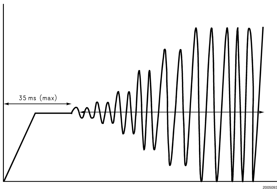
FIGURE 2. Fade-In Behavior
