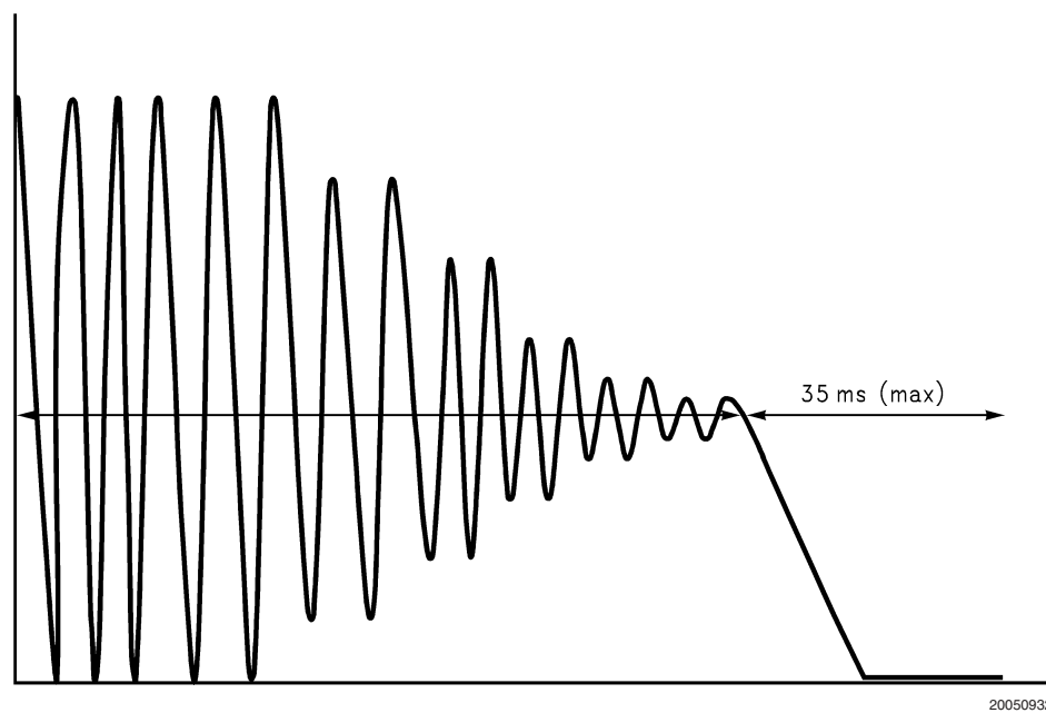
FIGURE 3. Fade-Out Behavior
