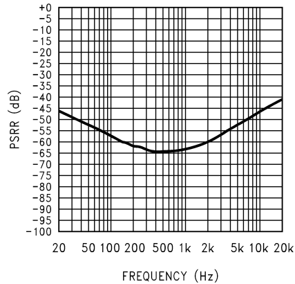
Power Supply Rejection Ratio (PSRR), V_{DD} = 2.6V
