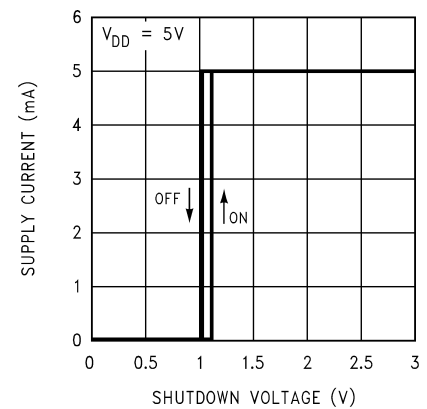
Shutdown Hysteresis Voltage V_{DD} = 5\text{V}
