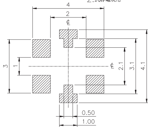
Recommand PCB Layout
