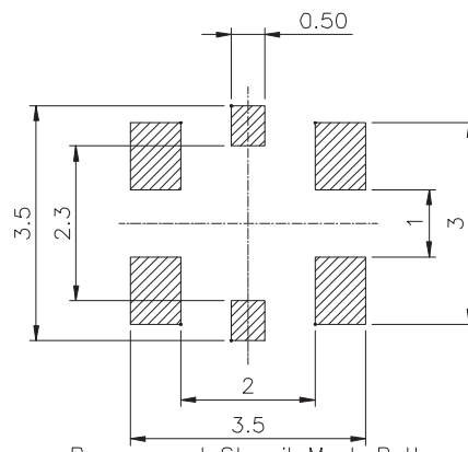
Recommand Stencil Mask Pattern (Mask Thickness 0.10~0.12mm)
