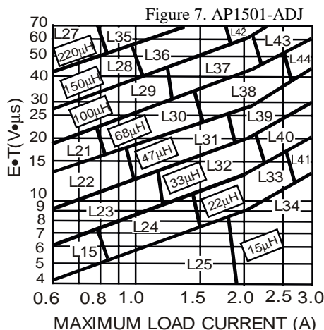
Figure 7. AP1501-ADJ
