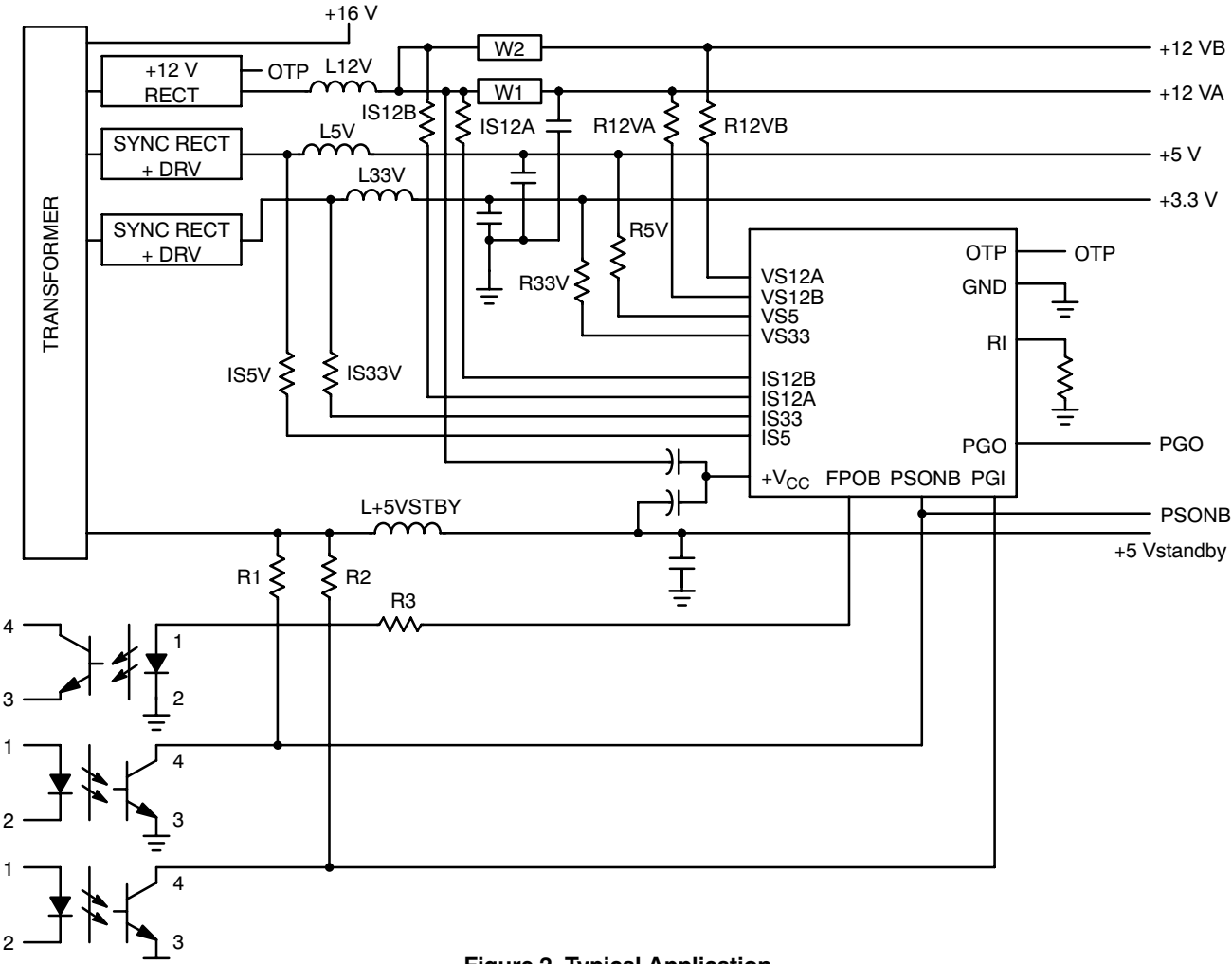
Figure 2. Typical Application
