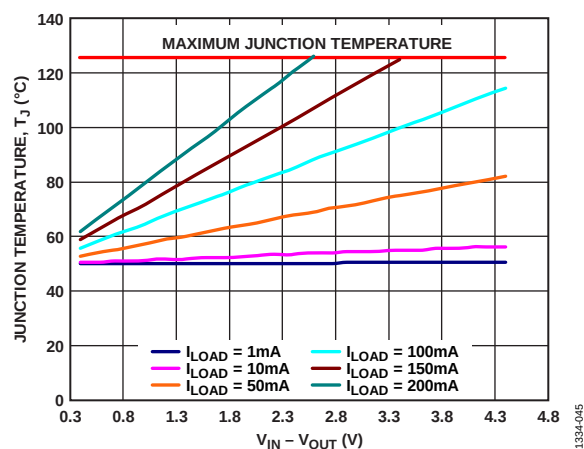
Figure 47. TSOT, 100 mm² of PCB Copper, T_A = 50^\circ\text{C}
