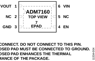
Figure 3. Pin Configuration, 6-Lead LFCSP
