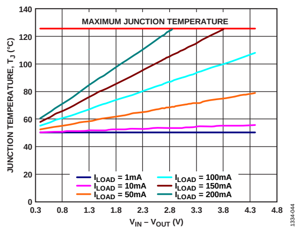
Figure 46. TSOT, 500 mm² of PCB Copper, T_A = 50^\circ\text{C}
