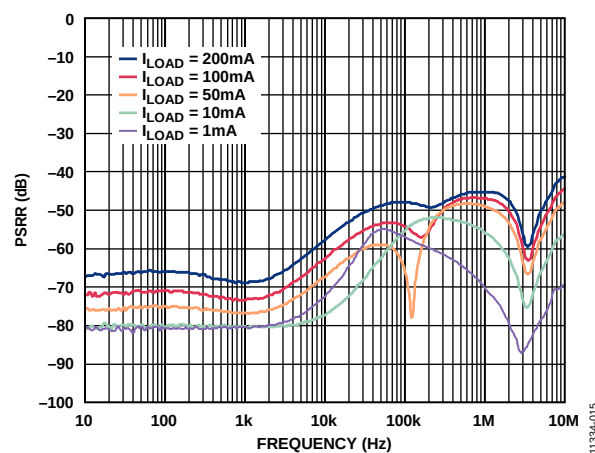
Figure 14. PSRR vs. Frequency and Load Current, 1 V Headroom, V_{OUT} = 1.8\text{ V}
