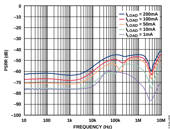
Figure 13. PSRR vs. Frequency and Load Current, 1 V Headroom, V_{OUT} = 2.5\text{ V}
