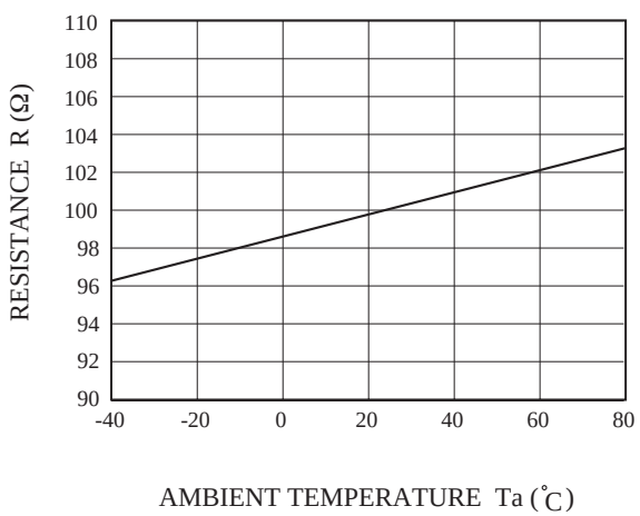
R_{Line} - TEMPERATURE
