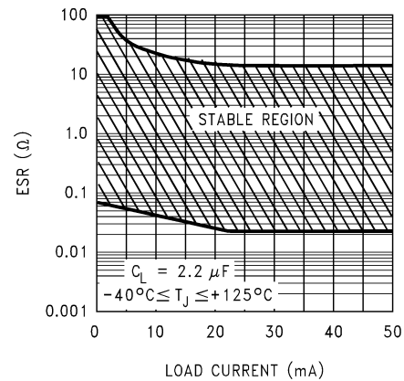
Figure 35. 2.2 \mu\text{F} ESR Range
