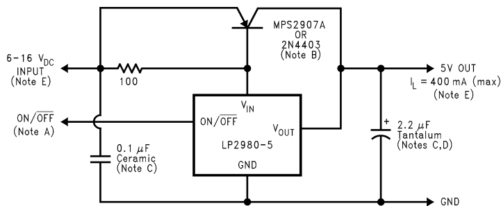
Figure 39. 5V/400mA Regulator
