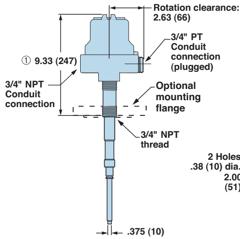
Integral Mount with Guarded Probe
