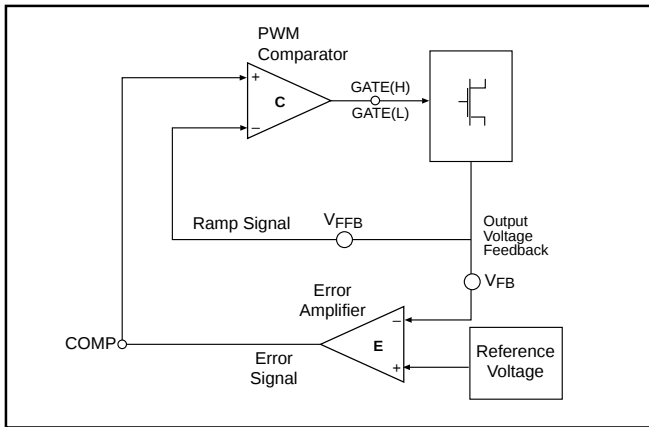
Figure 1: V 2 ™ Control Diagram.
