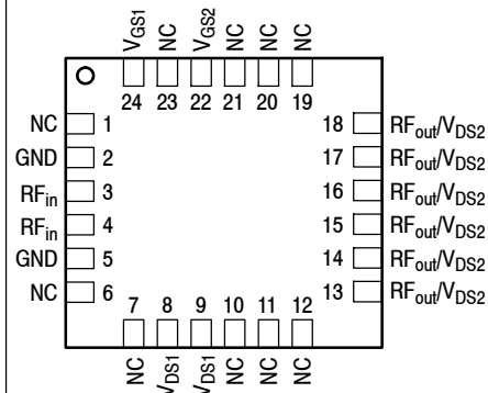
Figure 2. Pin Connections
