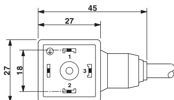
Valve connector, type AD
