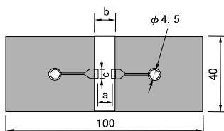
Fig.1 t : 1.6mm
