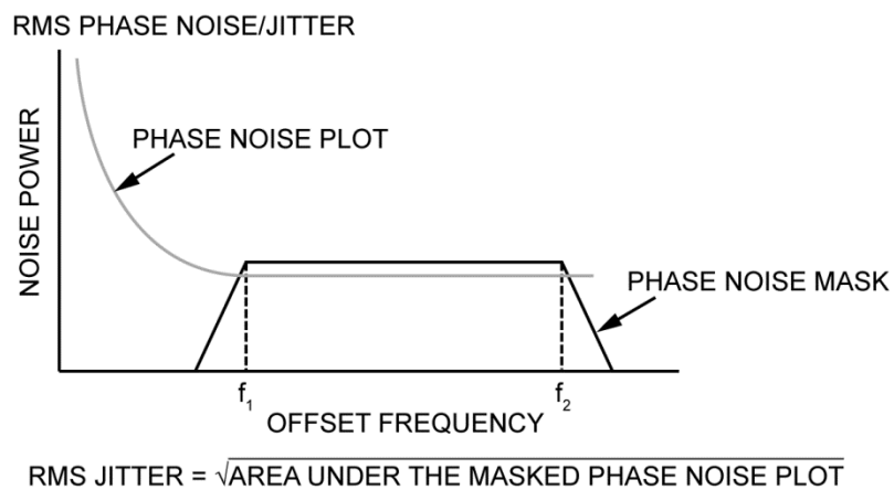
Figure 3. RMS Phase/Noise Jitter
