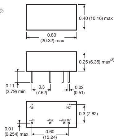
DIP Package
