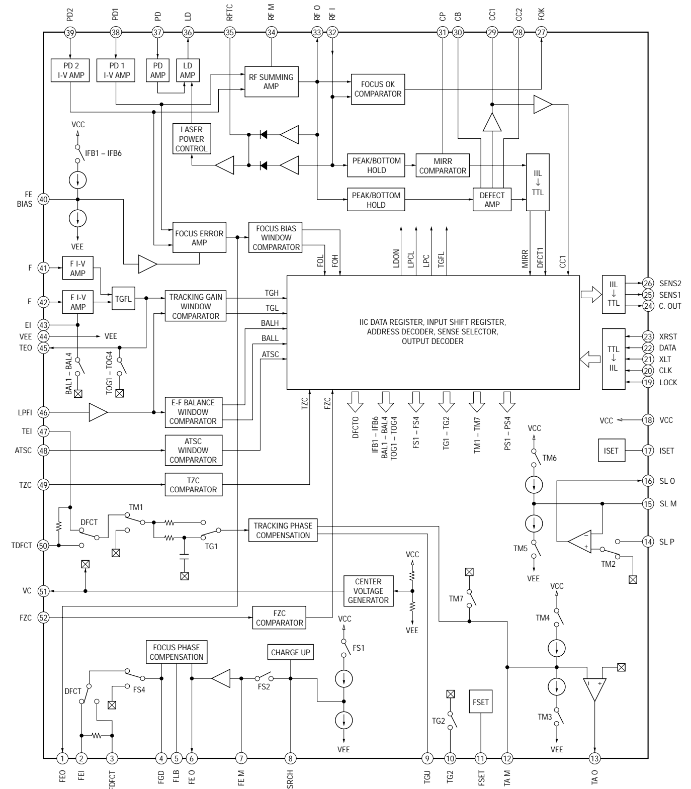
IC11 CXA1992BR
