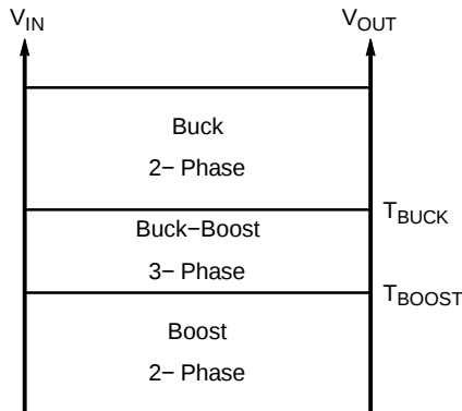
Figure 17. Conversion Mode
