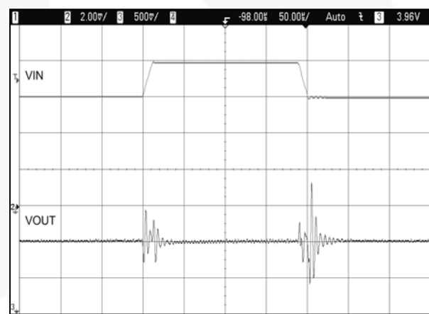
Figure 19. Line Transient V_{IN} = 3.7\text{ V} to 4.2\text{ V} , V_{OUT} = 2.5\text{ V} , 10\text{ }\Omega Load, 50\text{ }\mu\text{s/div} .
