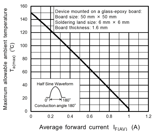
Fig. 10.4 T_{a(max)} - I_{F(AV)}
